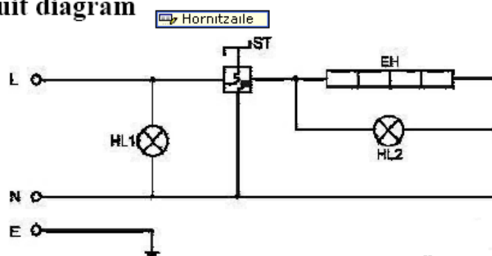
Fig 4. Circuit diagram of salamander with adjustable top
